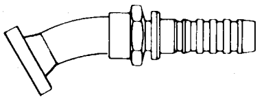
"O" Ring Flange- 22-1/2° (Code 61- SAE J518)
