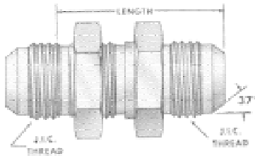
3905 STRAIGHT BULKHEAD UNION ADAPTER JIC Thread To JIC Bulkhead Thread
