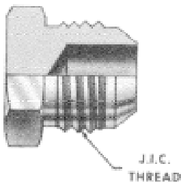
3105P J.I.C. FLARE TUBE PLUG Screw Into Nut To Plug Line
